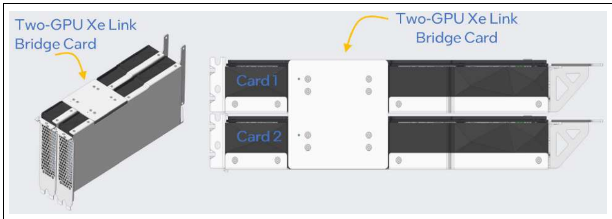
Figure 3-3. Two-Card Configuration Numbering with Intel X e Link Physical Bridge Installed
