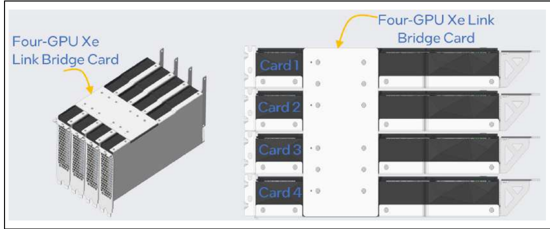
Figure 3-6. Four-Card Configuration Numbering with Intel X e Link Physical Bridge Installed
